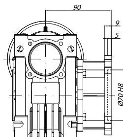
FA - SHORT FLANGE
